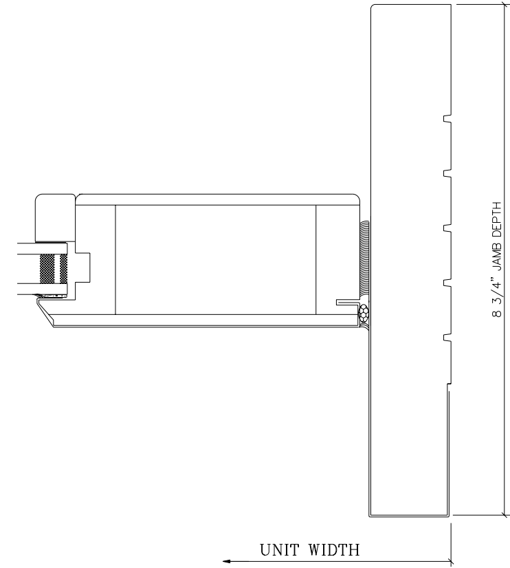
2 LIFT-SLIDE JAMB FULL SCALE
